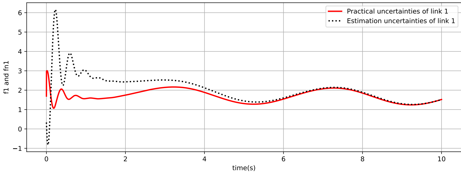
Disturbance Estimation Performance ( S=3 , S1=2 , m=5 )
